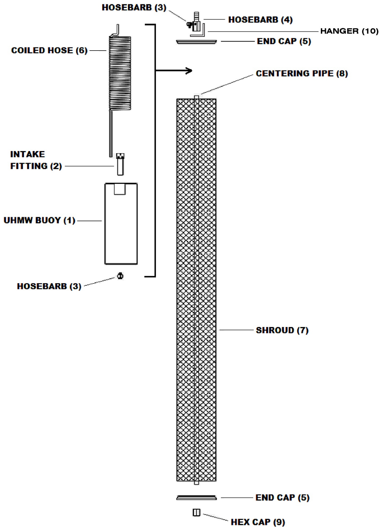
Figure 8-6: 4" High Temperature, Heavy Oil Skimmer Assembly, extended options available
