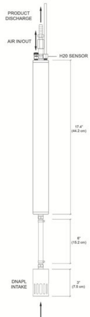
Figure 1-3: DNAPL recovery configuration for Stainless Steel Pump
